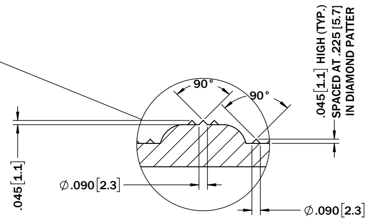
DETAIL C
